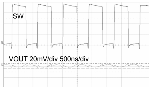
Heavy Load Operation ( V_{out}=1.8V , I_o=200mA )
