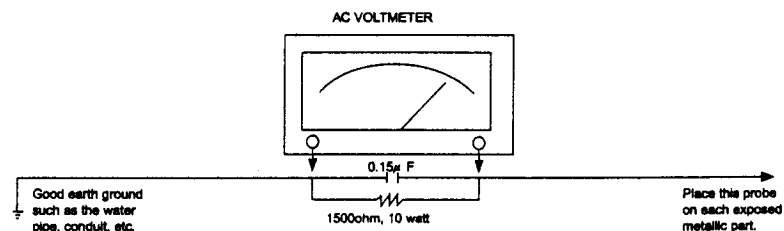
Figure 1.AC Leakage Current Check
