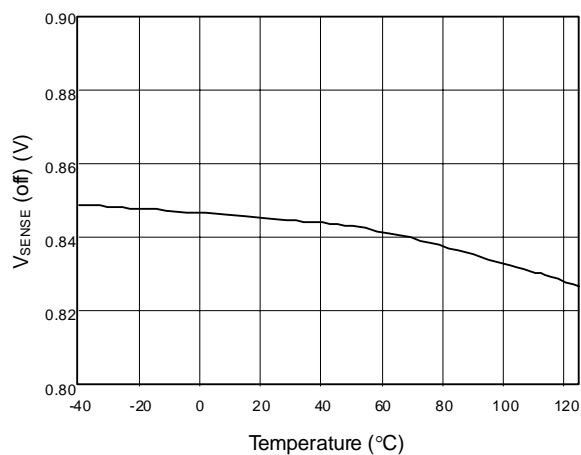
Fig. 2 V SENSE (off) vs. Temperature
