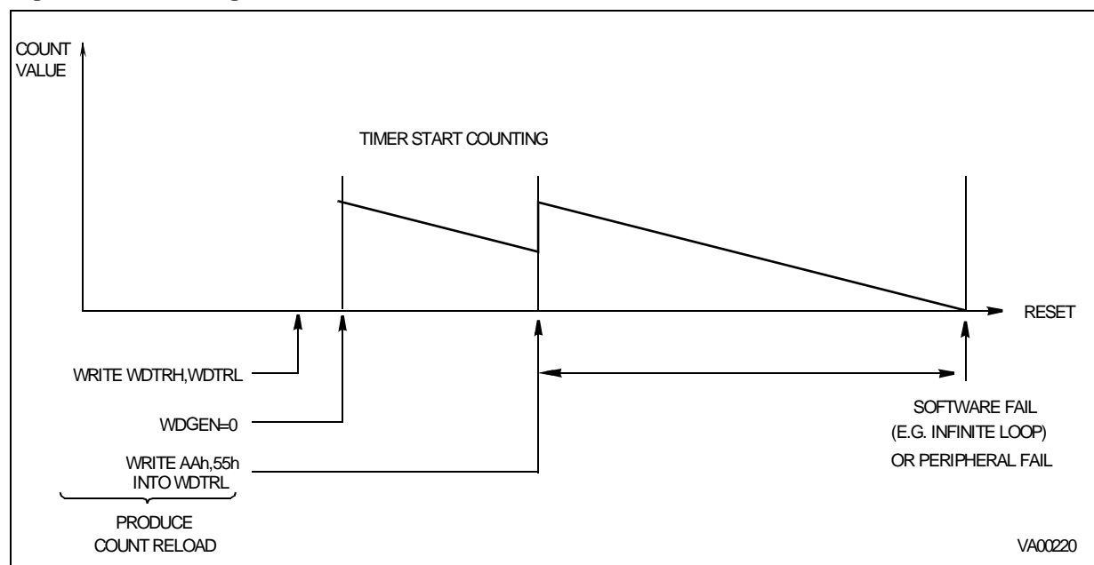
Figure 44. Watchdog Timer Mode
