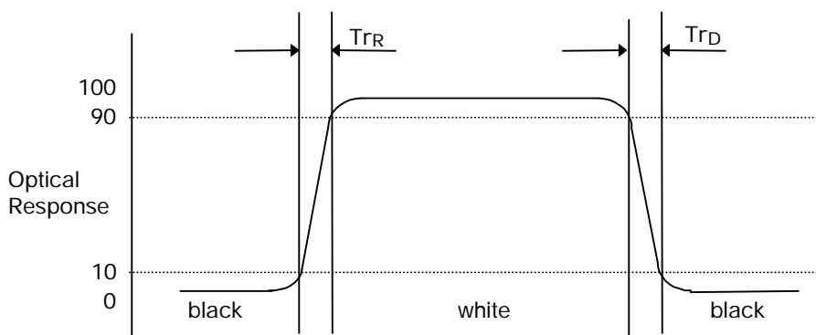
FIG. 3 Response Time
