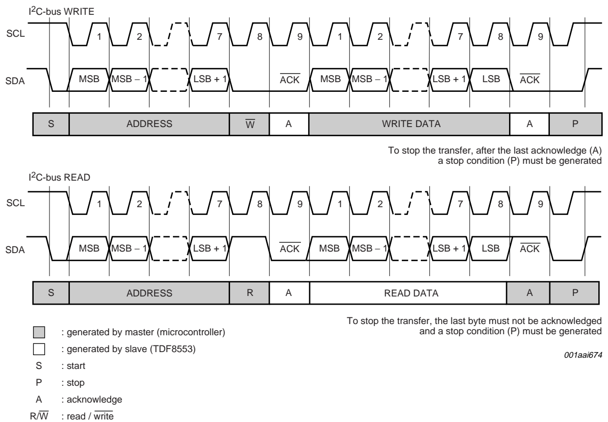
Fig 10. I 2 C-bus read and write modes
