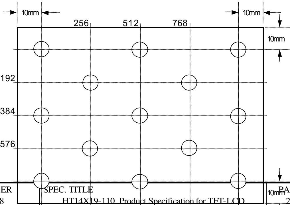
Figure 3. Uniformity Measurement Locations (13 points)
