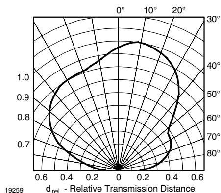
Figure 13. Vertical Directivity
