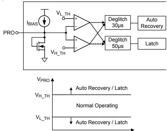
Figure 4. PRO Pin Diagram
