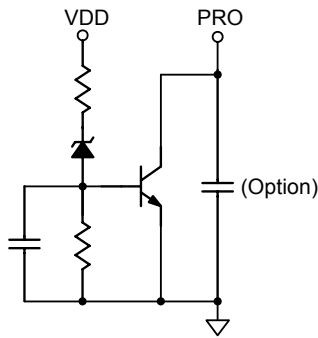
Figure 7. For VDD OVP
