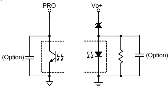
Figure 8. For V OUT OVP
