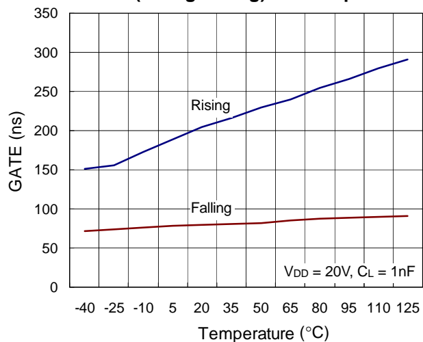
GATE (Rising/Falling) vs. Temperature
