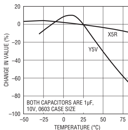
Figure 4. Ceramic Capacitor Temperature Characteristics
