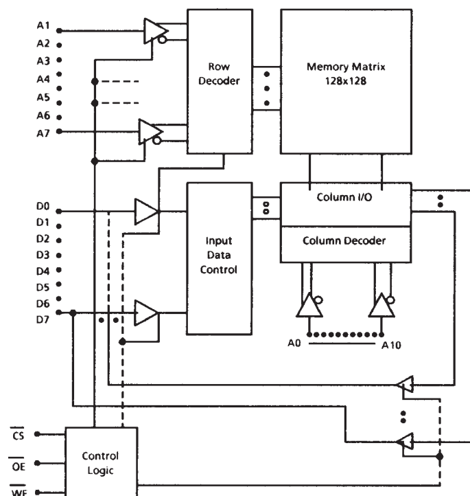
Figure 2: Block Diagram
