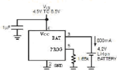
600mA Single Cell Li-Ion Charger
