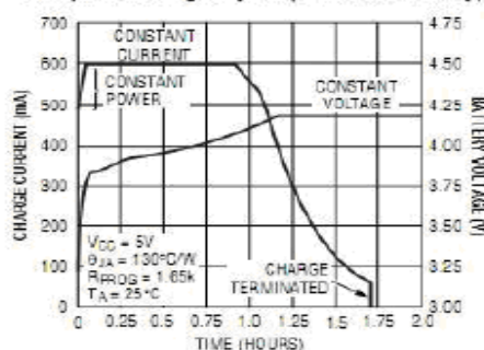
Complete Charge Cycle (750mAh Battery)
