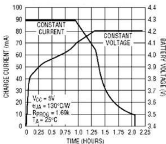
Complete Charge Cycle(130mAh Battery)
