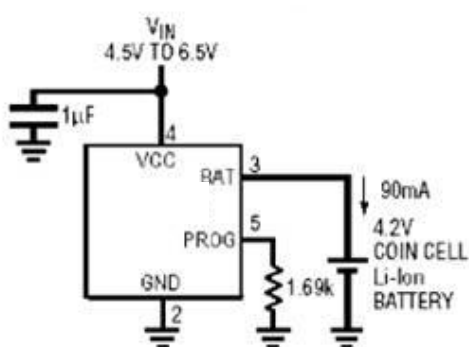
90mA Single Cell Li-Ion Charge
