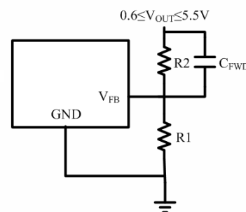
Figure 2. Setting the WD1013EA Output Voltage
