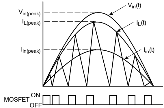
Figure 28. Inductor Waveform During CrM Operation
