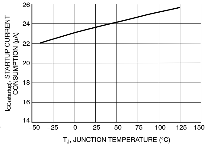
Figure 22. Startup Current Consumption vs. Junction Temperature
