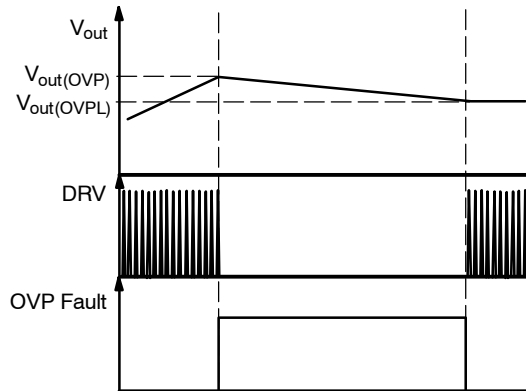
Figure 43. OVP Operation
