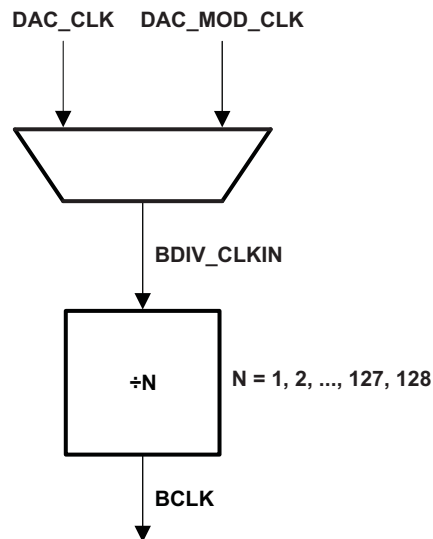
Figure 5-21. BCLK Output Options
