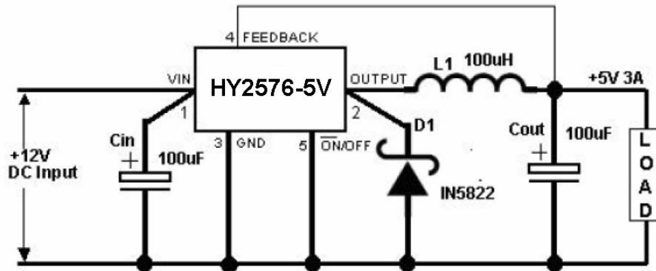
Figure 12. Typical Application of HY2576 For 5V
