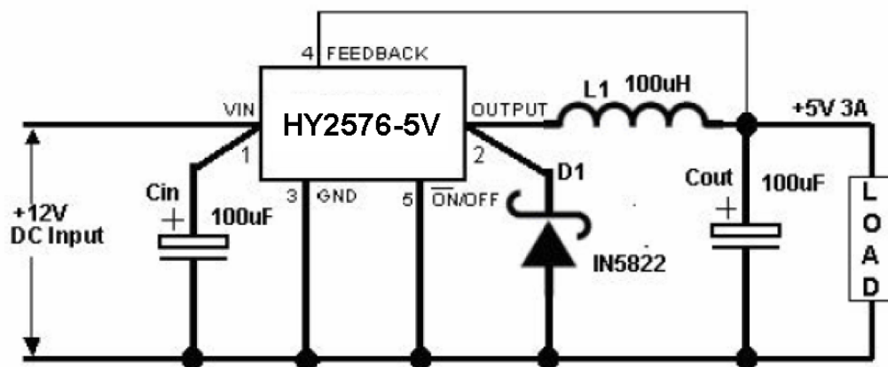
Figure 3. Typical Application of HY2576
