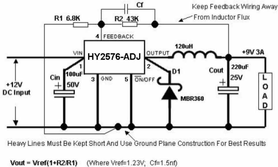
Figure 13. Typical Application of HY2576 For ADJ
