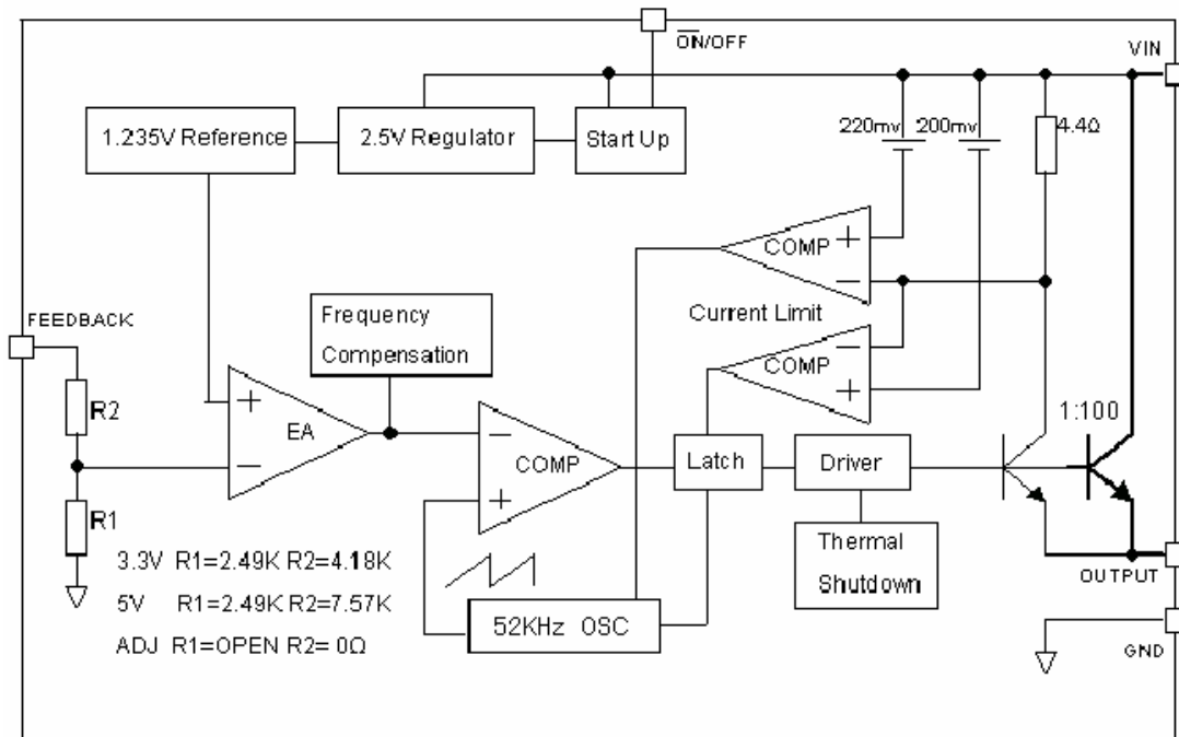
Figure 2. Functional Block Diagram of HY2576
