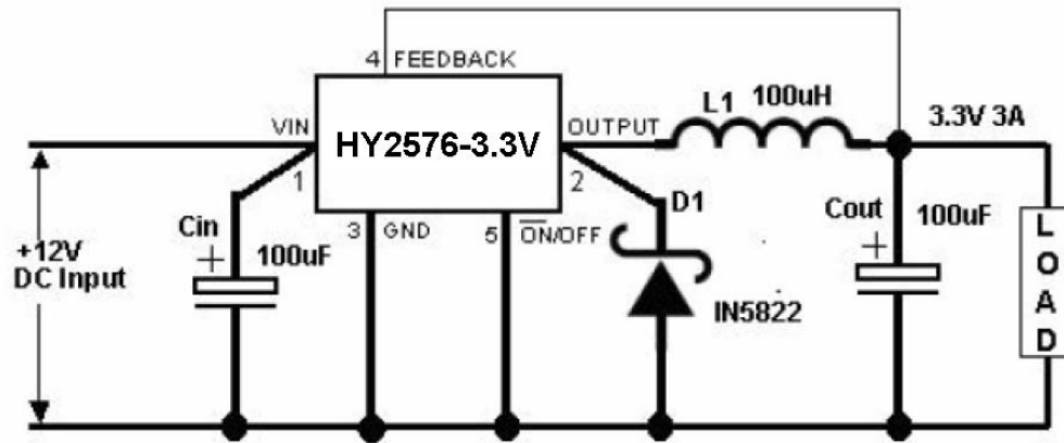
Figure 11. Typical Application of HY2576 For 3.3V
