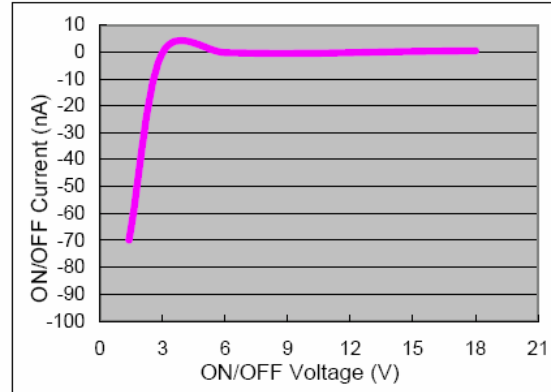
FSP3124 ON/OFF Current v.s. ON/OFF Voltage ( V_{in}=12V )
