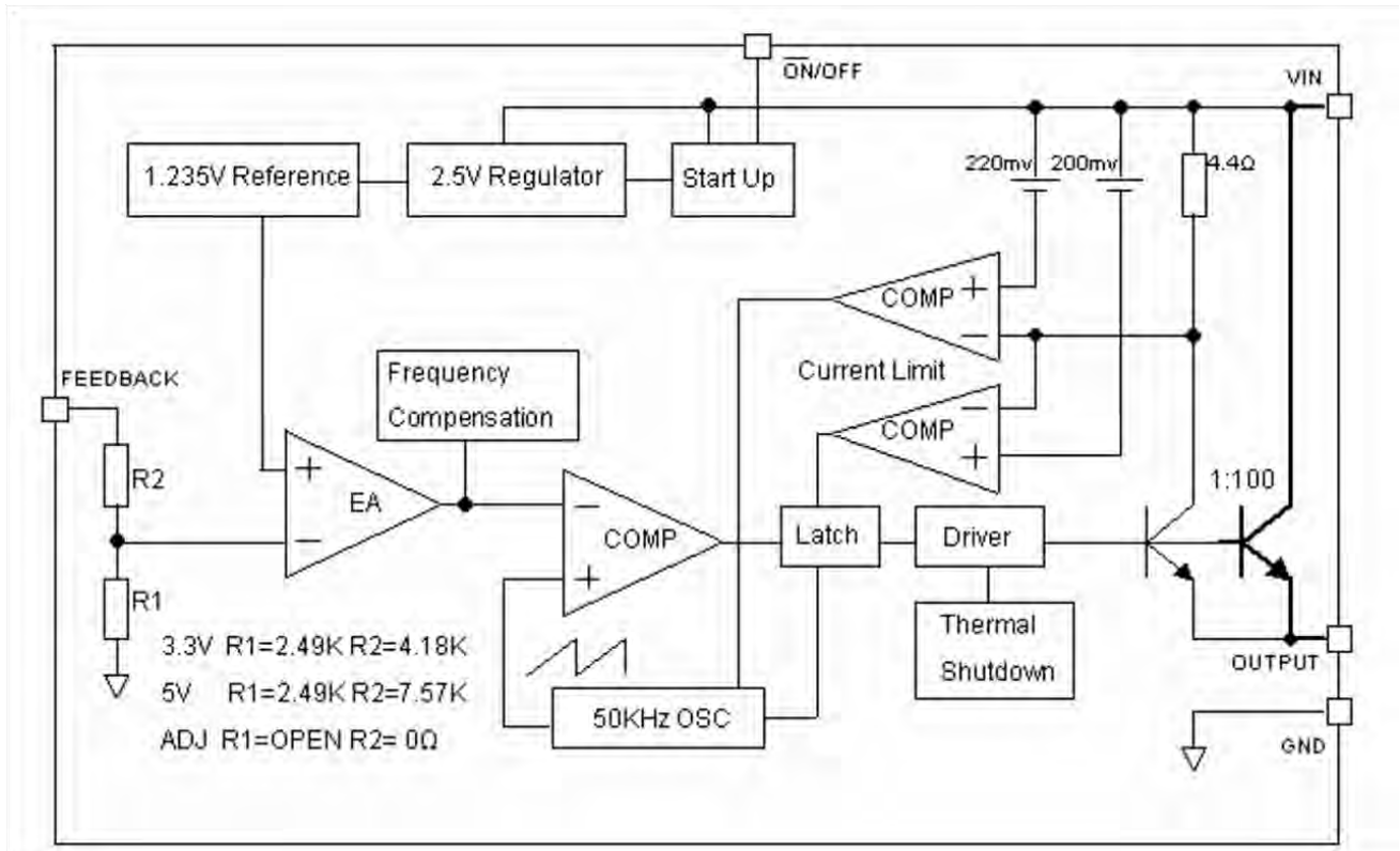
Figure 2. Functional Block Diagram of FAC2576
