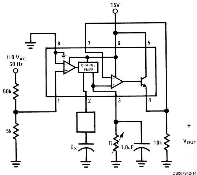
Capacitance Meter V_{OUT} = 1V-10V for C_X = 0.01 to 0.1 mFd (R = 111k)
