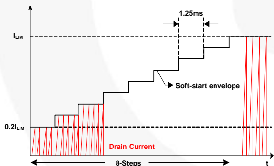
Figure 25. Internal Soft-Start
