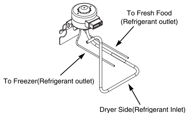
3 way valve
