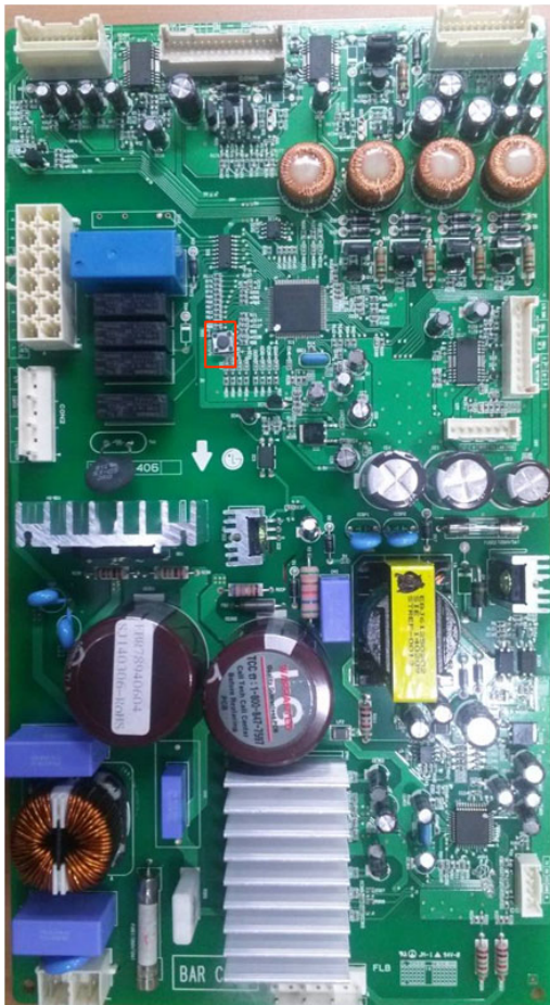
Main PCB
