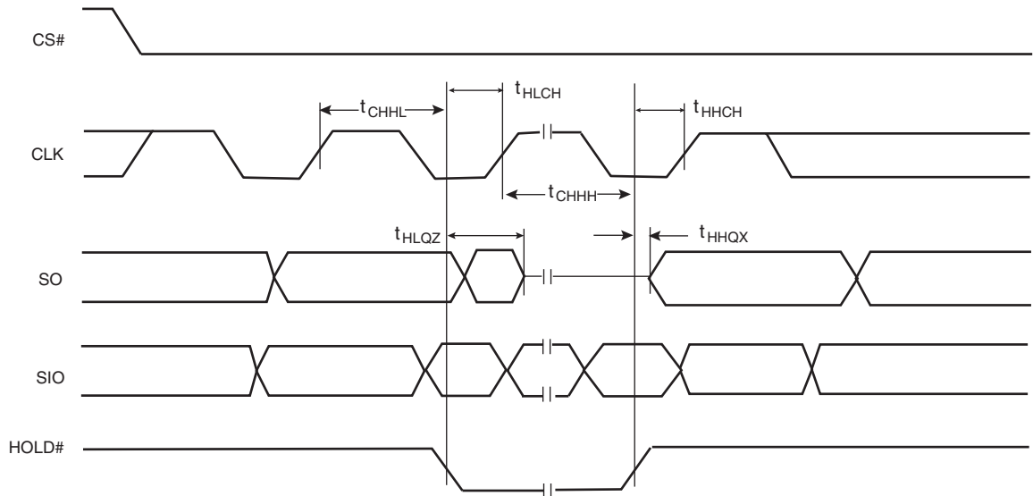
Figure 8.5 Hold Timing
