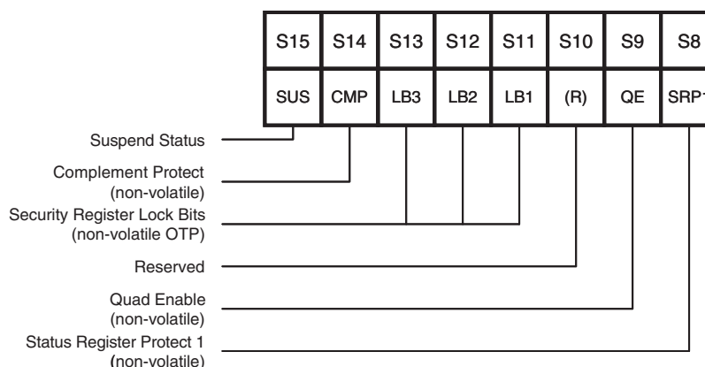
Figure 6.2 Status Register 2
