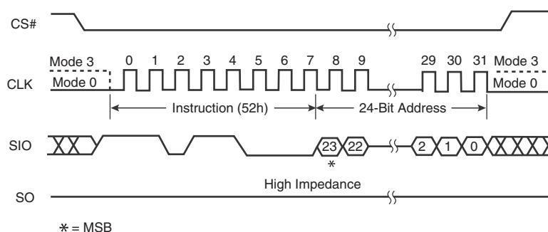
Figure 7.23 32 KB Block Erase Instruction Sequence Diagram
