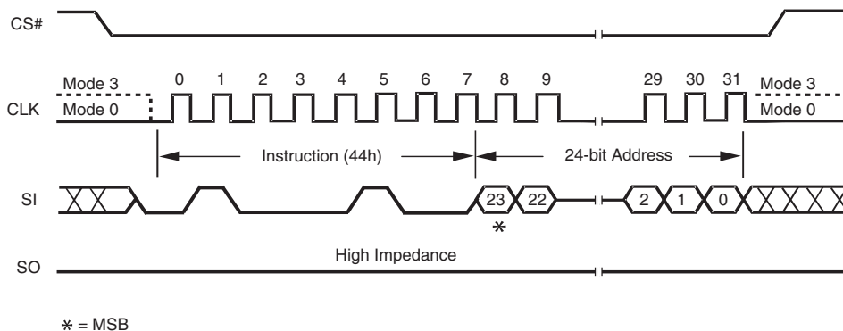
Figure 7.37 Erase Security Registers Instruction Sequence
