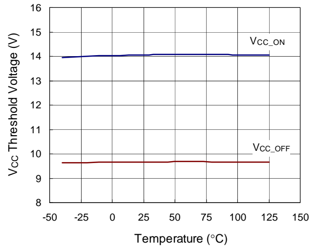
V CC Threshold Voltage vs. Temperature
