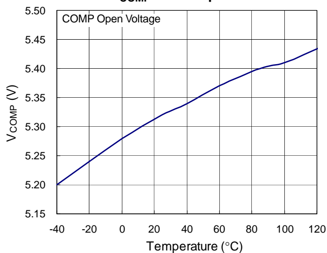
V COMP vs. Temperature
