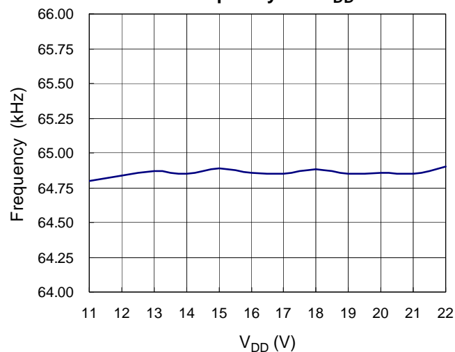
Frequency vs. V DD
