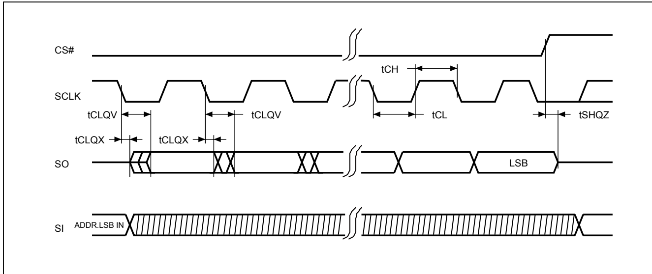
Figure 43. Output Timing
