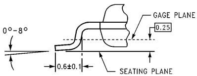
DETAIL A TYPICAL, SCALE: 40X
