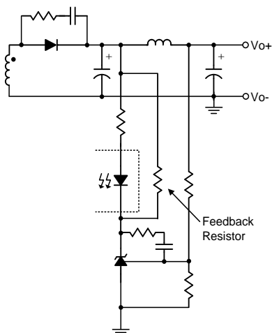
Figure 10. Feedback Resistor
