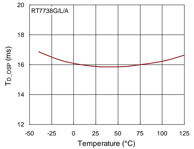
T D_OSP vs. Temperature
