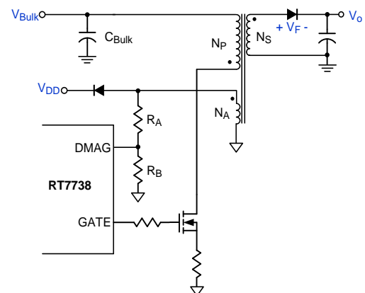
Figure 5. Design DMAG Pin Resistance
