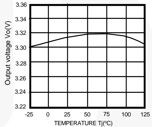
Figure 6. Output Voltage vs. Temperature ( T_j )
