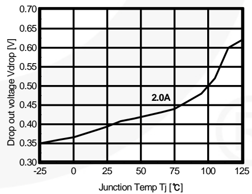
Figure 8. Dropout Voltage vs. Junction Temperature
