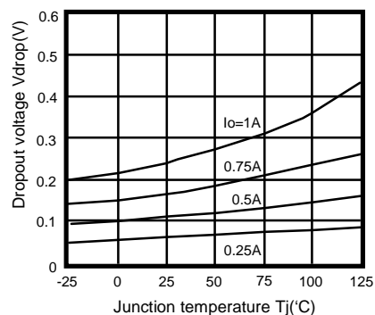
FIG.6 Dropout Voltage vs. Junction Temperature
