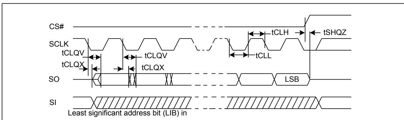
Figure 44. Output Timing Diagram
