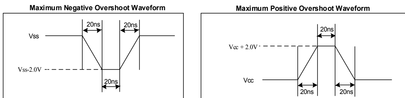
Figure 41. Maximum Negative/positive Overshoot Diagram
