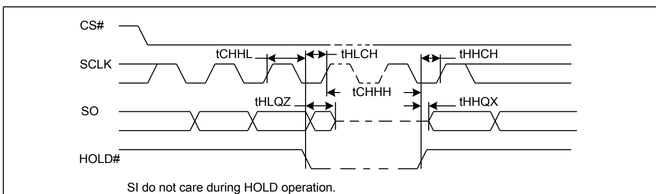
Figure 46. Hold Timing Diagram
